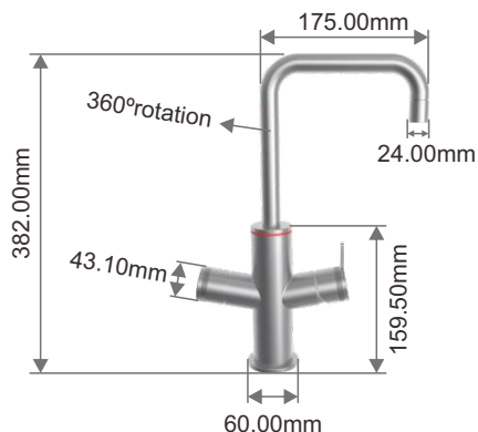
UNITO Boiler
